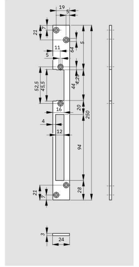
FLM 24-94
