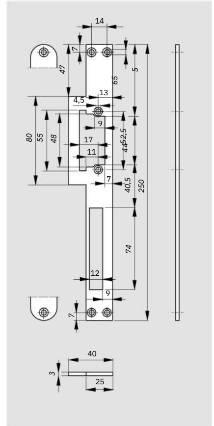
FLR 25 / FLM 25
