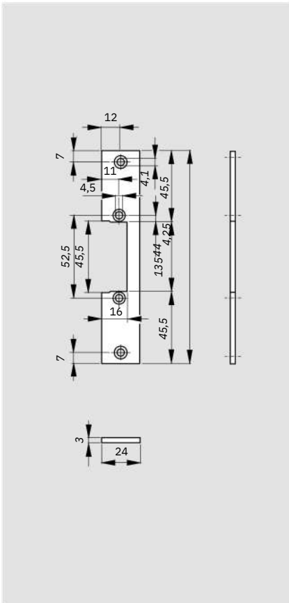
FKH 24
