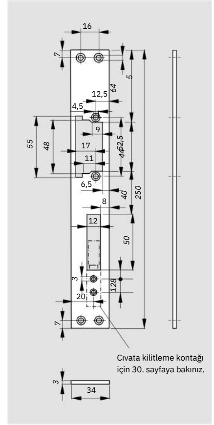
FLM 34-RK
