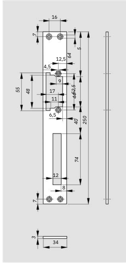
FLM 34
