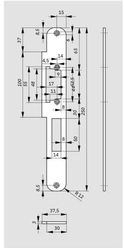
FLR 30
