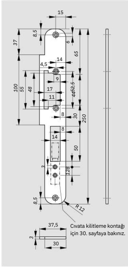
FLR 30-RK
