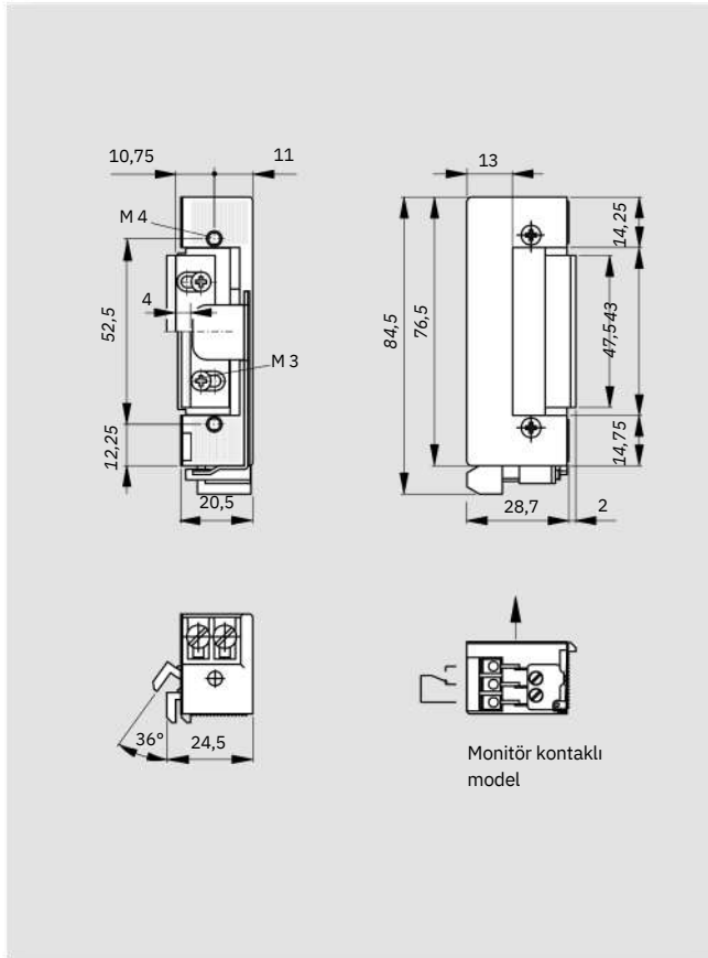
Fire 447 / Fire 448
